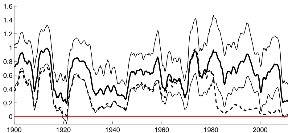
Figure 5: Counterfactual experiment: Median and 68% central posterior bands for \hat{b}_f for fixed VAR model coefficients ( \mathbf{A}_{1976.1} ). The dashed line represents the median of \hat{b}_f without fixing the VAR model coefficients.
