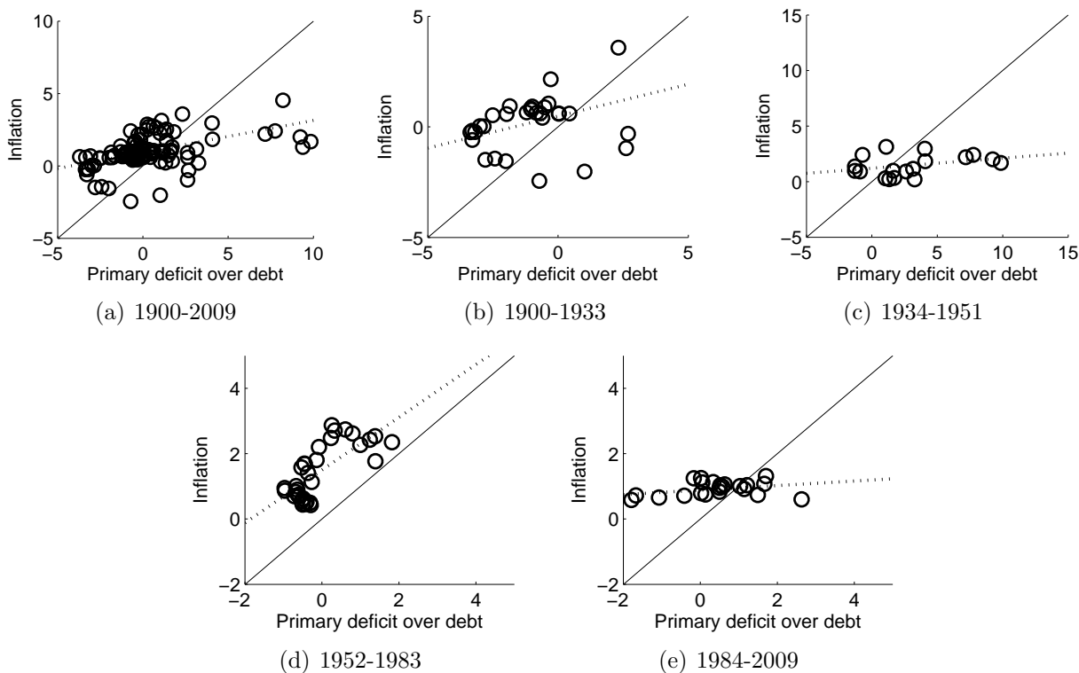
Figure 2: Scatter plots of filtered time series ( \beta = 0.95 ) of inflation and primary deficits over debt. The dashed line indicates the slope of the scatter and the solid line is the 45° line.
