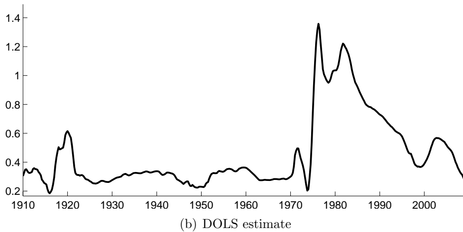
Figure 15: Rolling sample (fixed window) regression coefficients.
