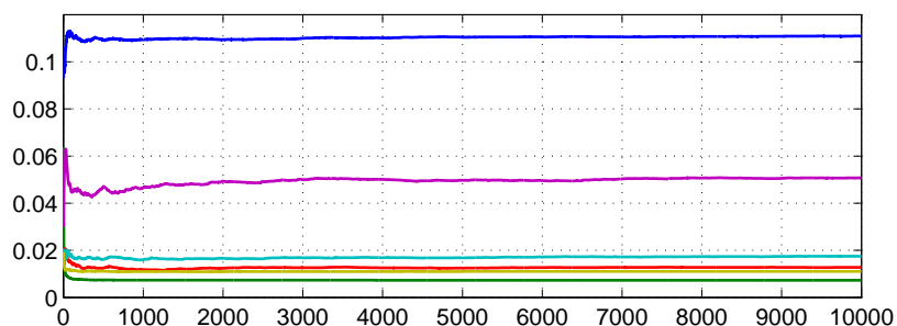
Figure 8: Running Mean Plot.
