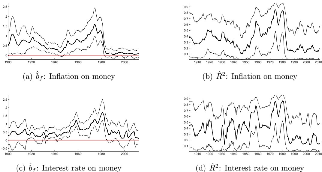
Figure 16: Selected low-frequency relationships.
