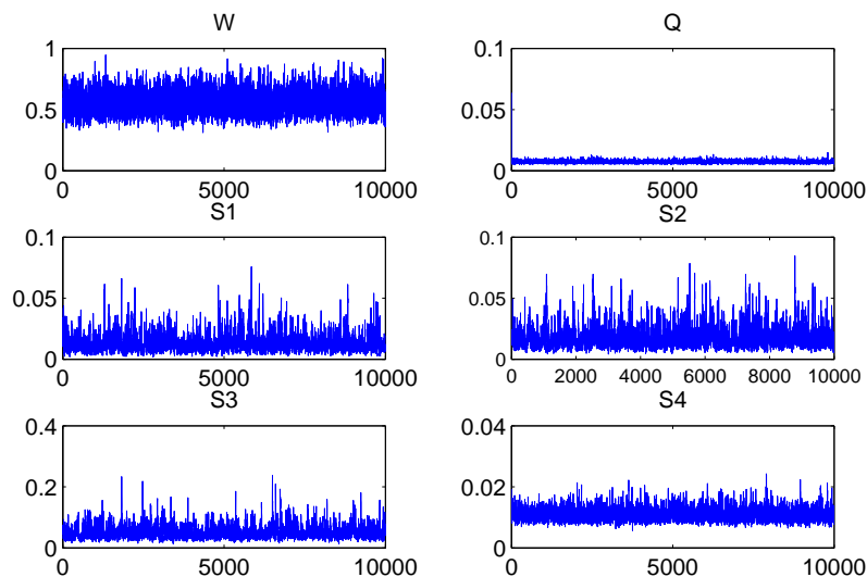
Figure 9: Trace Plot.
