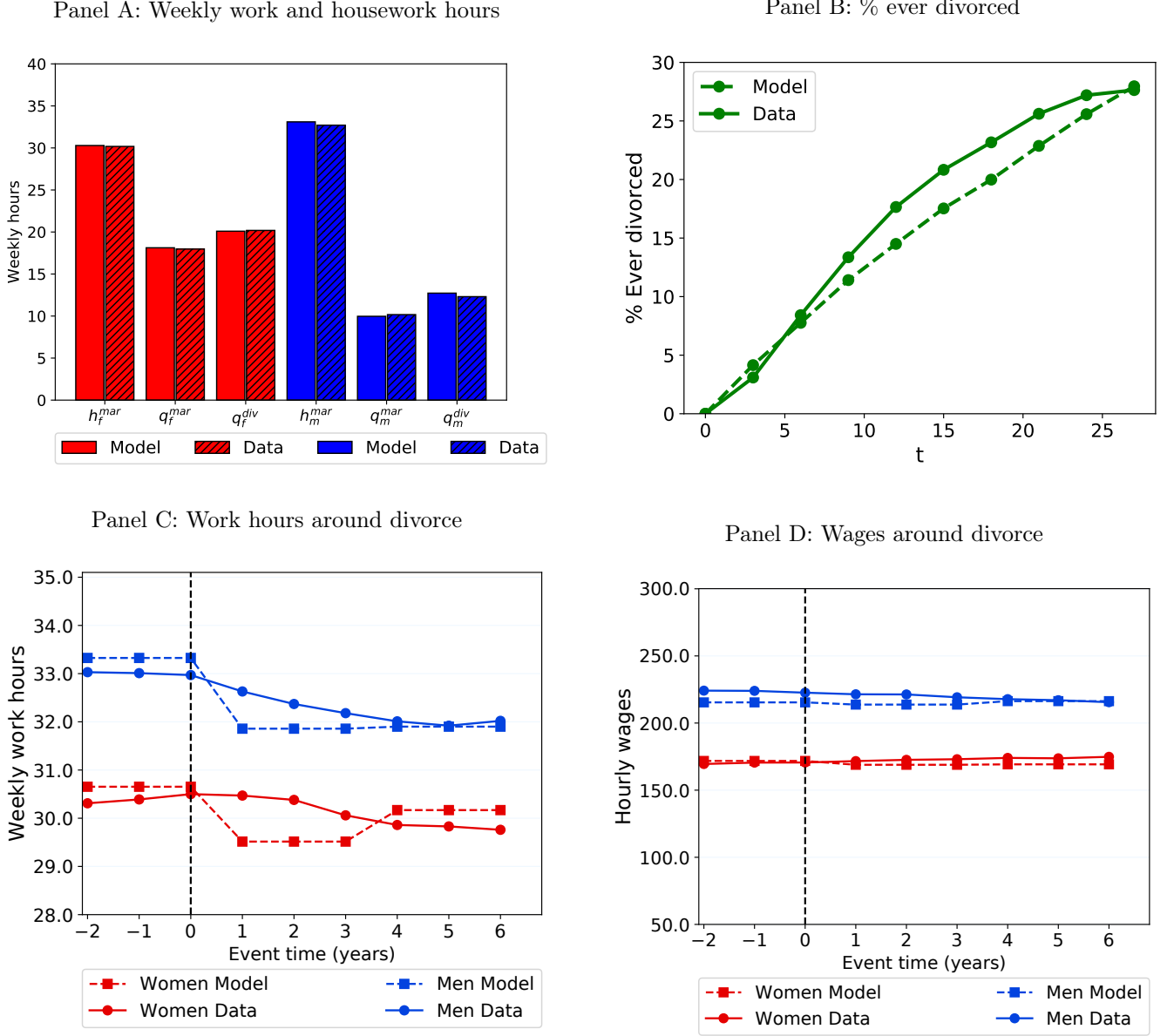
FIGURE 8: Model fit
