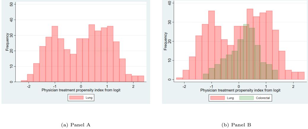
Figure 3: Physician heterogeneity
