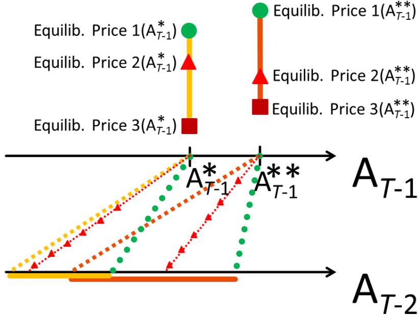
Figure 9: Consistent equilibrium beliefs for different successor states A_{T-1} .
